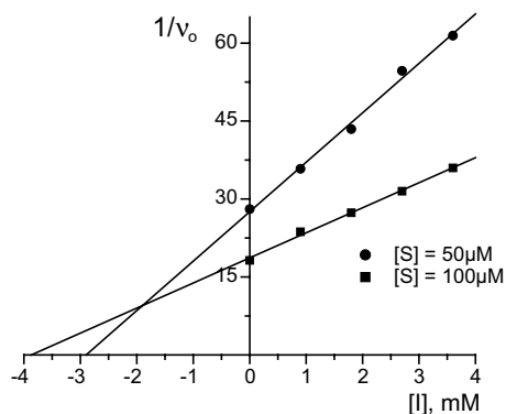
Figure 1. The Dixon plot for the inhibition of carboxypeptidase A by (RS)-2.
