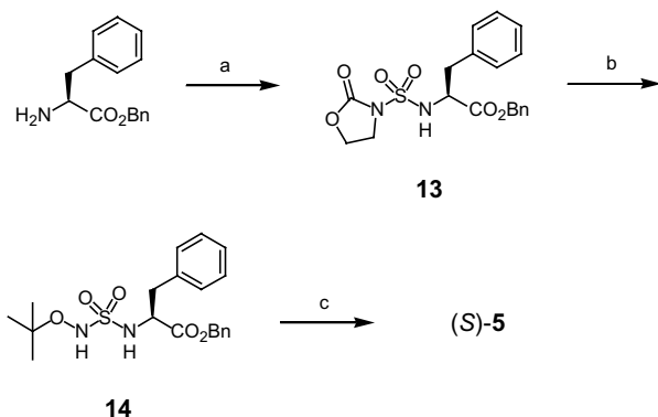
Scheme 3. Reagents, conditions, and yield: (a) N -(chloroethyl)sulfamoyl chloride, Et 3 N, CH 2 Cl 2 , rt, 12 h, 95%; (b) t BuONH 2 ·HCl, Et 3 N, MeCN, reflux, 12 h, 49%; (c) (i) TiCl 4 (1.5 equiv), CH 2 Cl 2 , rt, 30 min; (ii) H 2 , Pd–C, MeOH, rt, 2 h, 37%.
