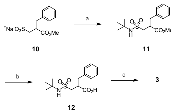
Scheme 2. Reagents, conditions, and yield: (a) (i) PCl 5 , toluene, rt, 2 h; (ii) t -BuNH 2 (3 equiv), toluene, 0 °C, 1 h, 71.5%; (b) 2 N NaOH, MeOH, rt, 12 h, 52.3%; (c) TFA, rt, 12 h, 95%.
