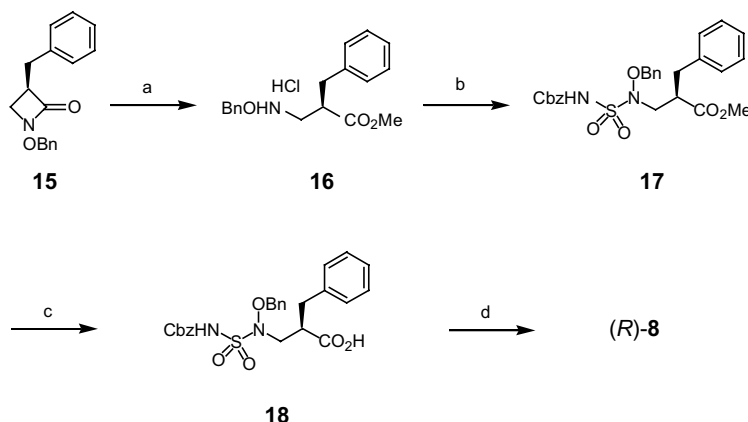
Scheme 4. Reagents, conditions, and yield: (a) TMSCl (4 equiv), MeOH, rt, 4 h, 98%; (b) CbzNH 2 SO 2 Cl prepared from OCNSO 2 Cl and BnOH (CH 2 Cl 2 , 0 °C, 30 min), Et 3 N, CH 2 Cl 2 , rt, 6 h, 88%; (c) LiOH (2 equiv), MeOH/H 2 O (3:1), rt, 2 h, 93%; (d) H 2 , Pd–C, MeOH, rt, 2 h, 95.5%.
