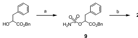
Scheme 1. Reagents, conditions, and yield: (a) (i) formic acid (1.5 equiv), chlorosulfonyl isocyanate (1.5 equiv), 0 °C, 4 h; (ii) ( S )-phenyllactic acid, pyridine (1.5 equiv), 0 °C, 12 h; 57%; (b) H 2 , Pd-C, MeOH, rt, 2 h, 99%.
